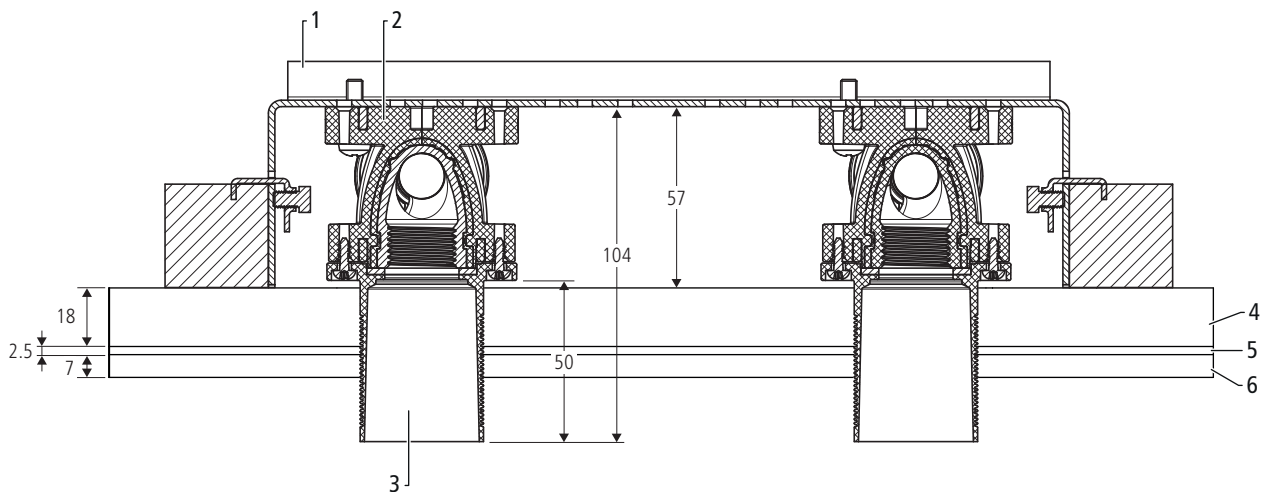
Fig. 11: Module GIS Optiflex, parement simple 18 mm 85121/84221
