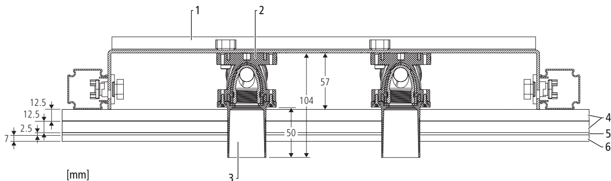
Fig. 13: Module Optiflex-Optivis, parement double 84214/85214
