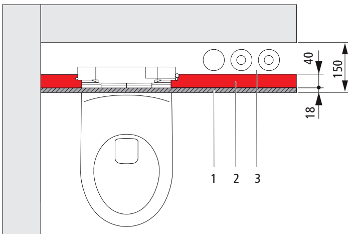
Abb. 22: Optivis-Tec-Vorwand 150 mm
