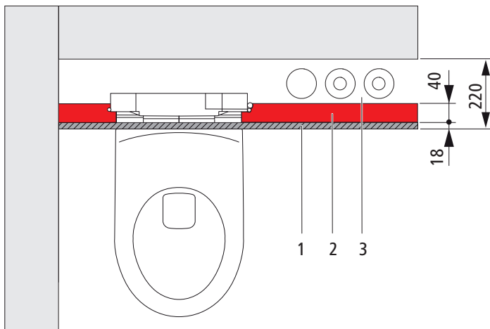
Abb. 23: Optivis-Tec-Vorwand 220 mm
