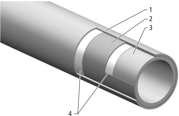
Fig. 58: Tubo Optiflex-Flowpress multistabile.
