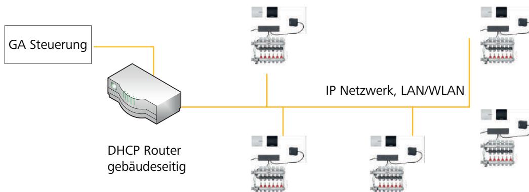
Abb. 7: Installationstopologie
