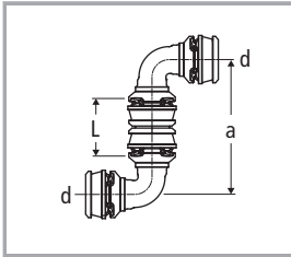
Coude 90° Optiflex-Flowpress 84240
