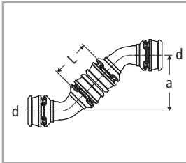
Coude 45° Optiflex-Flowpress 84241
