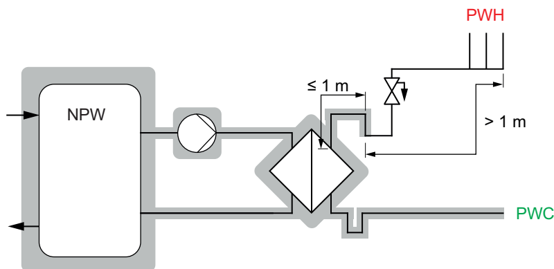
Fig. 20: Station ECS
