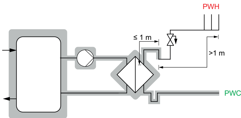
Fig. 20: Station ECS instantanée
